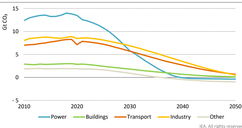
Figure 3.1 ▶ CO 2 emissions by sector in the NZE
